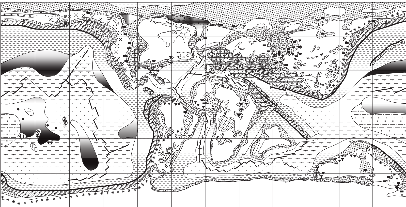
Fig. 2. The lithologic–paleogeographic map for the Santonian Age of the Late Cretaceous (symbols as in Fig. 1).
